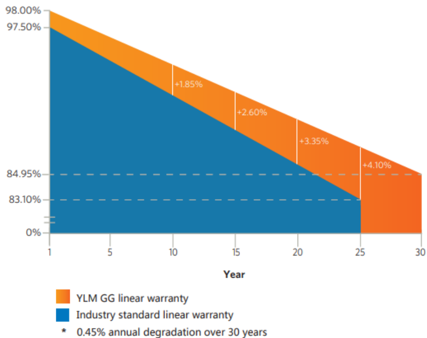
Figure 2: Power warranty for p-type mono-Si GLASS/GLASS modules
